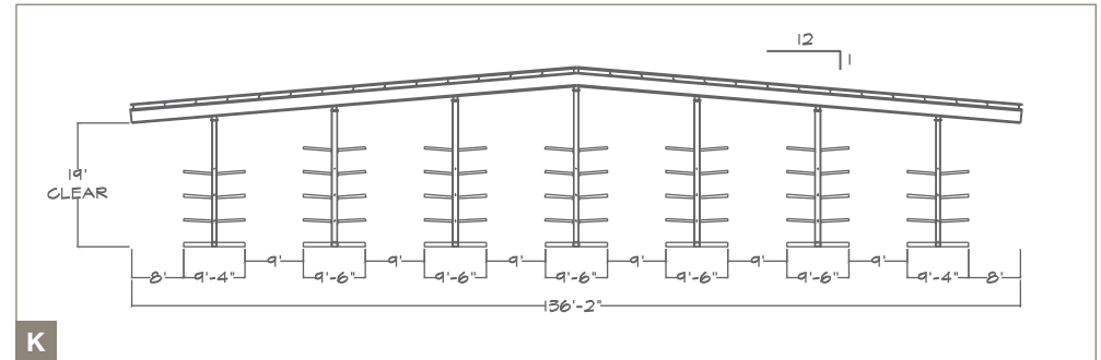
Narrow-Aisle Drive-Thru Building (for side loading forklifts)
