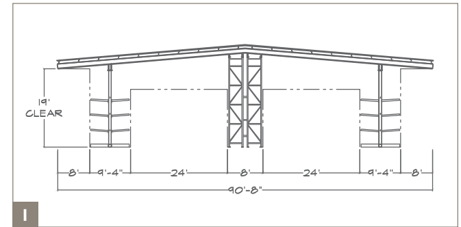
Multi-Purpose Double-Aisle Building
