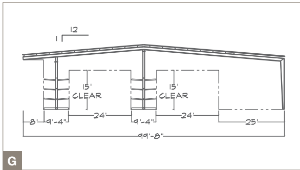
Double-Aisle Cantilever / Bulk Storage Building
