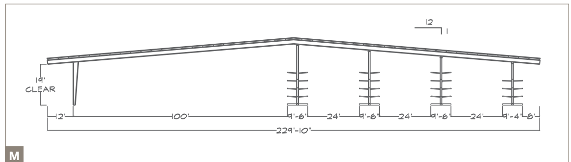
Multi-Purpose Clear Span Drive-Thru Building
