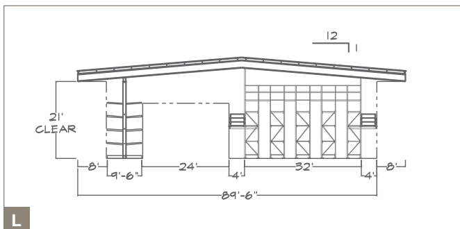
Single-Aisle Power Bin Building
