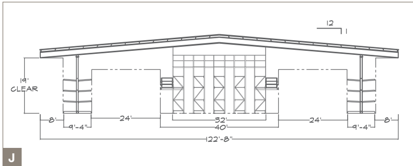
Double-Aisle Power Bin Building
