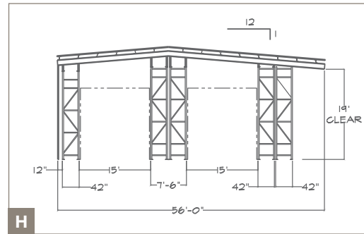
Double-Aisle Pallet Rack Warehouse
