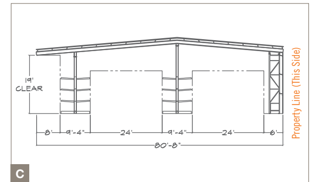
C Double-Aisle Property Line Building
