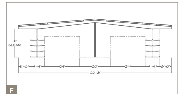
F Double-Aisle Cantilever Building
